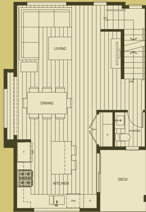
MAIN 600 SQFT
